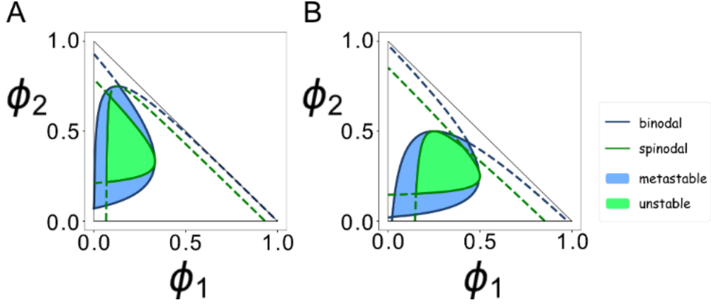
Figure. 5: Ternary phase diagrams. (A) \chi_{1-2} = 0 ; \chi_{1-3} = 8 ; \chi_{2-3} = 3 ; (B) \chi_{1-2} = 0 ; \chi_{1-3} = 8 ; \chi_{2-3} = 4 .
