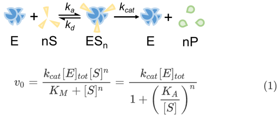
Figure. 2: Mathematical representation of typical enzymatic kinetic reaction.
