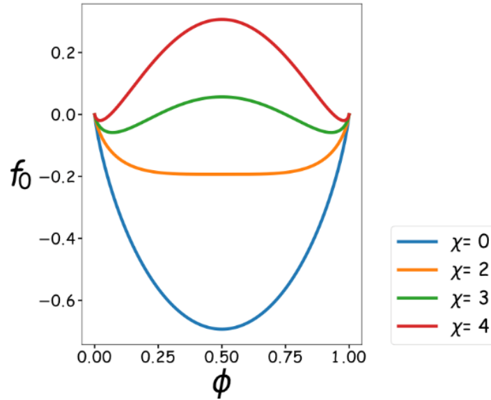
Figure. 2: Plot of the symmetric part of free energy density at various values of \chi .
