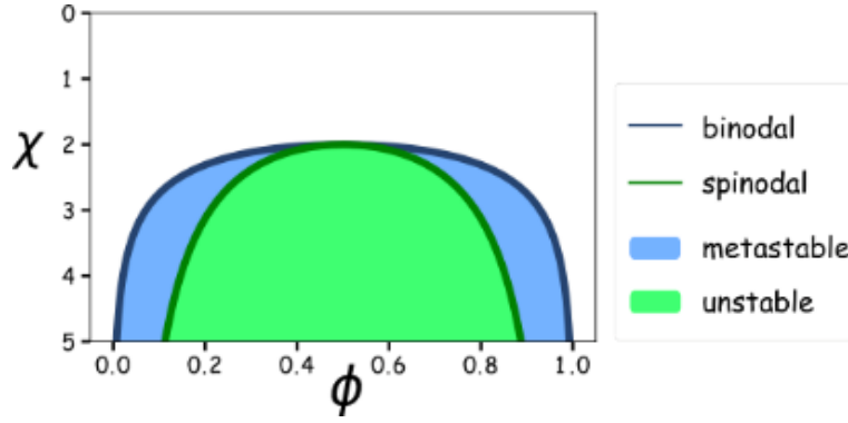
Figure. 4: Binary phase diagram. The binodal line shows the boundary between conditions under which phases can and cannot separate. The spinodal line shows the boundary between two different formations: spinodal decomposition and nucleation. The area confined by spinodal line is the unstable region while the area between the binodal line and spinodal line is the metastable region.
