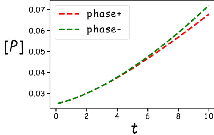
Figure. 6: The average product concentration over time. When substrate diffuses normally down the concentration gradient, the groups with and without phase separation show a slight difference.
