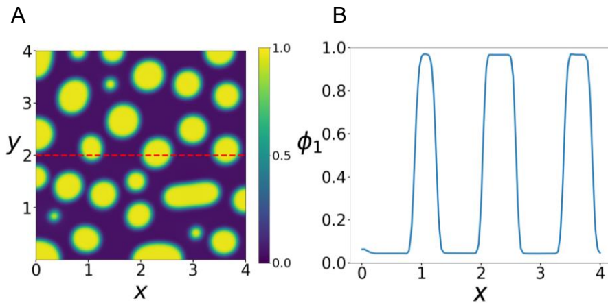
Figure. 6: Simulation for dynamic evolution of phase separation under \chi_{1-2} = 0 , \chi_{1-3} = 3 , \chi_{2-3} = 4 . (A) The concentration distribution of \phi_1 ; (B) The concentration of \phi_1 on the
