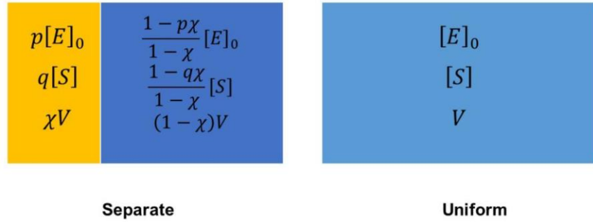
Figure. 1: Illustration of a dichotomous separate box and a uniform box.
