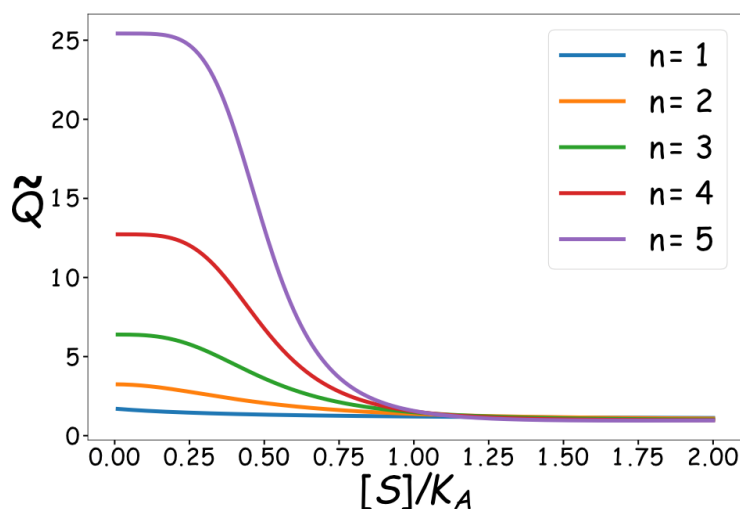
Figure. 4: Positive cooperative binding promotes the acceleration process. The calculation is conducted under the conditions \chi = 0.3 , p = 2.65 and q = 2 .
