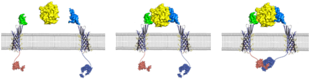
Figure 1 – Conceptual representation of our device. In the presence of a ligand (yellow), the mutual distance of the complementary signaling proteins (green and blue) will be reduced. The resulting proximity of the intracellular signaling protein domains (red and blue), results in the transduction of a signal.
