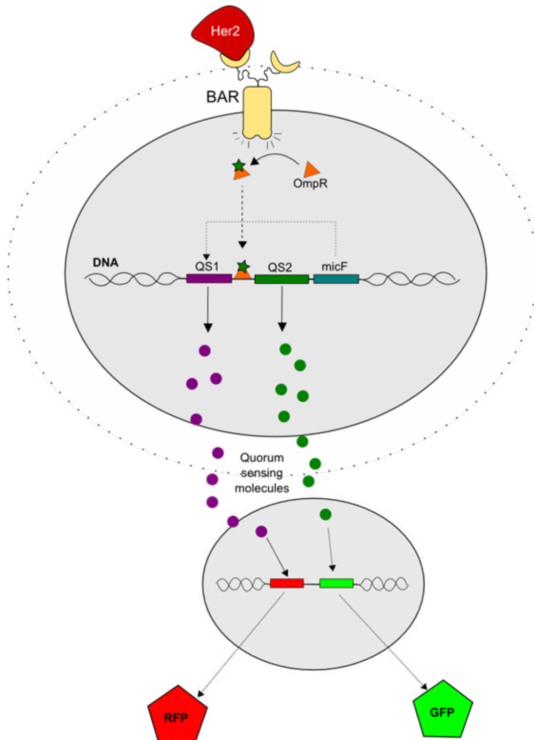
Figure 1: The Affibody-Based Bacterial Biomarker Assay (ABBBA), a novel tool for disease biomarker detection. The disease biomarker (here: Her2) can specifically and sensitively bind to the bacterial antigen receptor (BAR), a fusion protein consisting of an affibody binder molecule and a bacterial transmembrane domain, called EnvZ. The binding triggers the signal transduction into the cytoplasmic space allowing the phosphorylation of OmpR to OmpR-P which targets the promoter region of a genetic locus coding for two different Quorum Sensing Synthetases (QS1 and QS2) . These will be highly regulated by OmpR phosphorylation, and introduce a switch in quorum sensing molecule secretion allowing a fluorometric read-out in a read-out strain. Depending on the quorum sensing molecule in the medium it will produce either one of two fluorophores (RFP or GFP). This switch in fluorescence will give us a clear and definite positive read-out upon biomarker binding.
